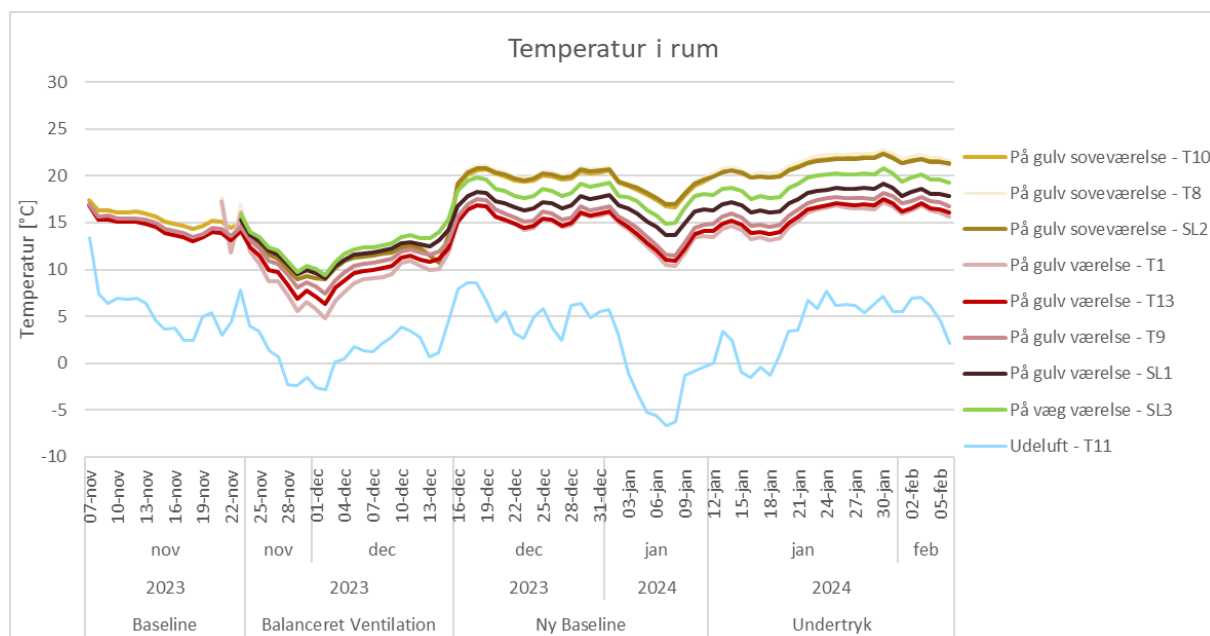
Figur 19: Temperatur for sensorer i rum
